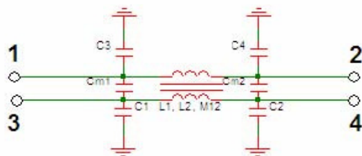
Figure 7: Lumped, Mutual Elements
