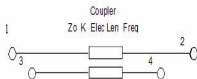
Figure 8: Distributed Model for Crosstalk
