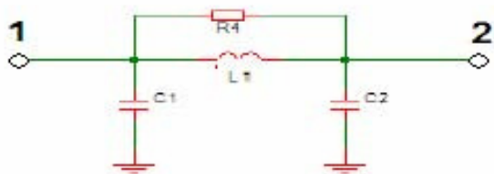
Figure 5: Lumped, Valid to <9GHz
